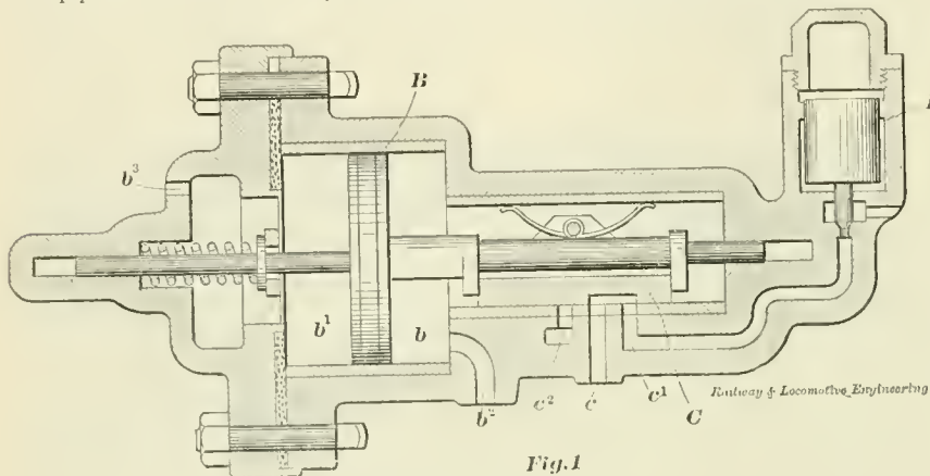
Fig. 1 AUTOMATIC RETAINING VALVE.
